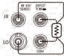
4W connection
